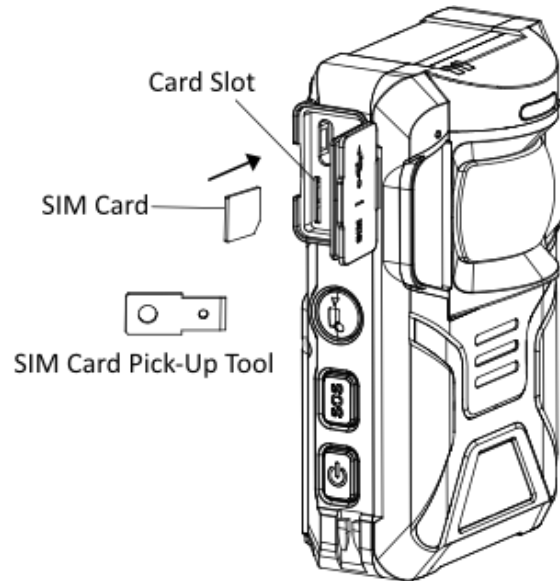
Figure 2-3 Install SIM Card
