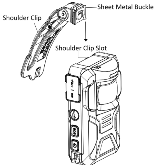
Figure 2-1 Install Shoulder Clip
